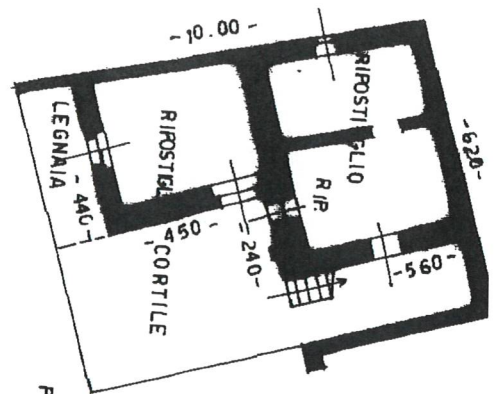
PIANO TERRA H 2.17
